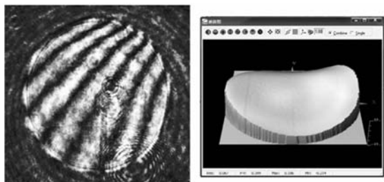
(a)RMS=λ/17,PV=λ/3,λ=630 nm,t=23℃
